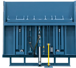
Vertical Storing Levelers
