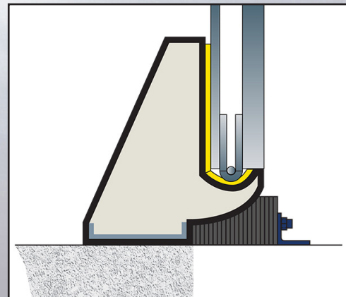
Trailer backed into position. (Truck In)
