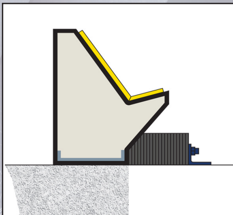
SEAL-TITE™ unique profile. (Top View Cross Section)
