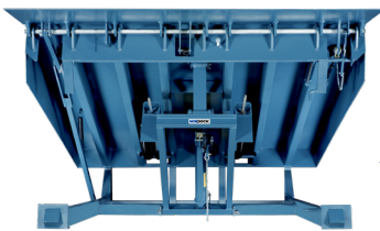
Mechanical Levelers
