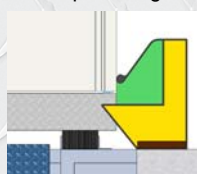
Wiper Seal for Trucks Equipped With Step or Tailgate
