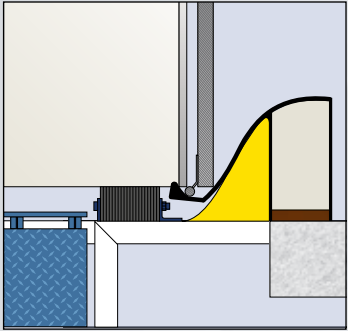
The optional Terminator™ Gap Seal automatically closes the opening left by the swing out trailer doors.
