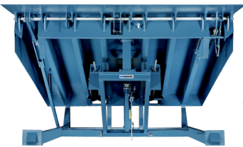
Mechanical Levelers
