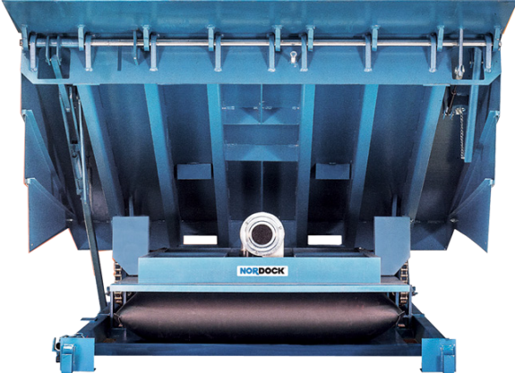
AIRDOCK® INDUSTRIAL™ (Model AD) The Model AD features the AUTO-DESCENT LIP™ Fully Yieldable Extension System, which uses the natural weight of the deck to activate the lip.
