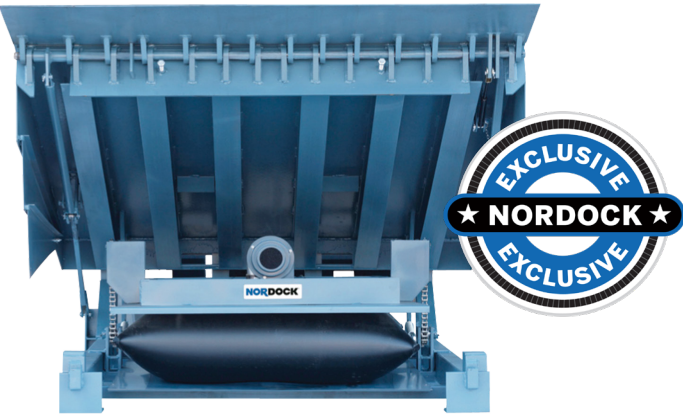
AIRDOCK® SUPER-DUTY™ (Model SA) The Model SA is the toughest air powered leveler ever built with a 60,000 lb. capacity.
