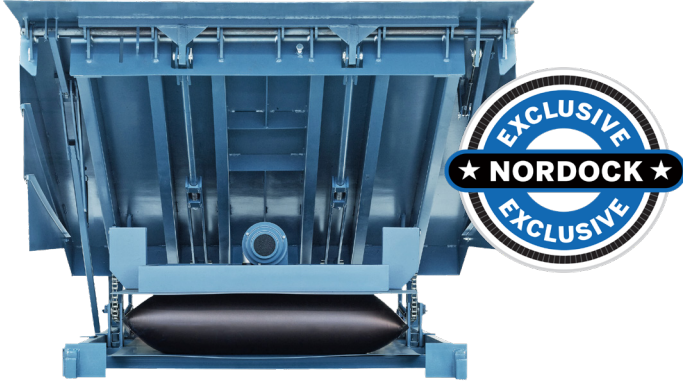
AIRDOCK® FLEX-LIP® (Model ADF) The Model ADF eliminates lip crown, providing the smoothest transition of any leveler on the market. Perfect for any warehouse this unique lip feature best accommodates industries processing or distributing fragile goods.
