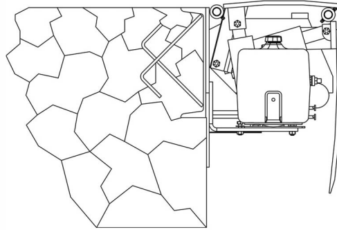
Side View – EFH Series
