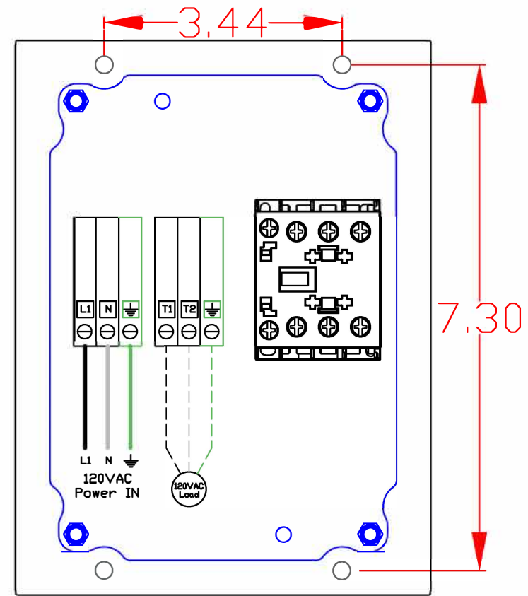
INTERNAL FRONT VIEW
